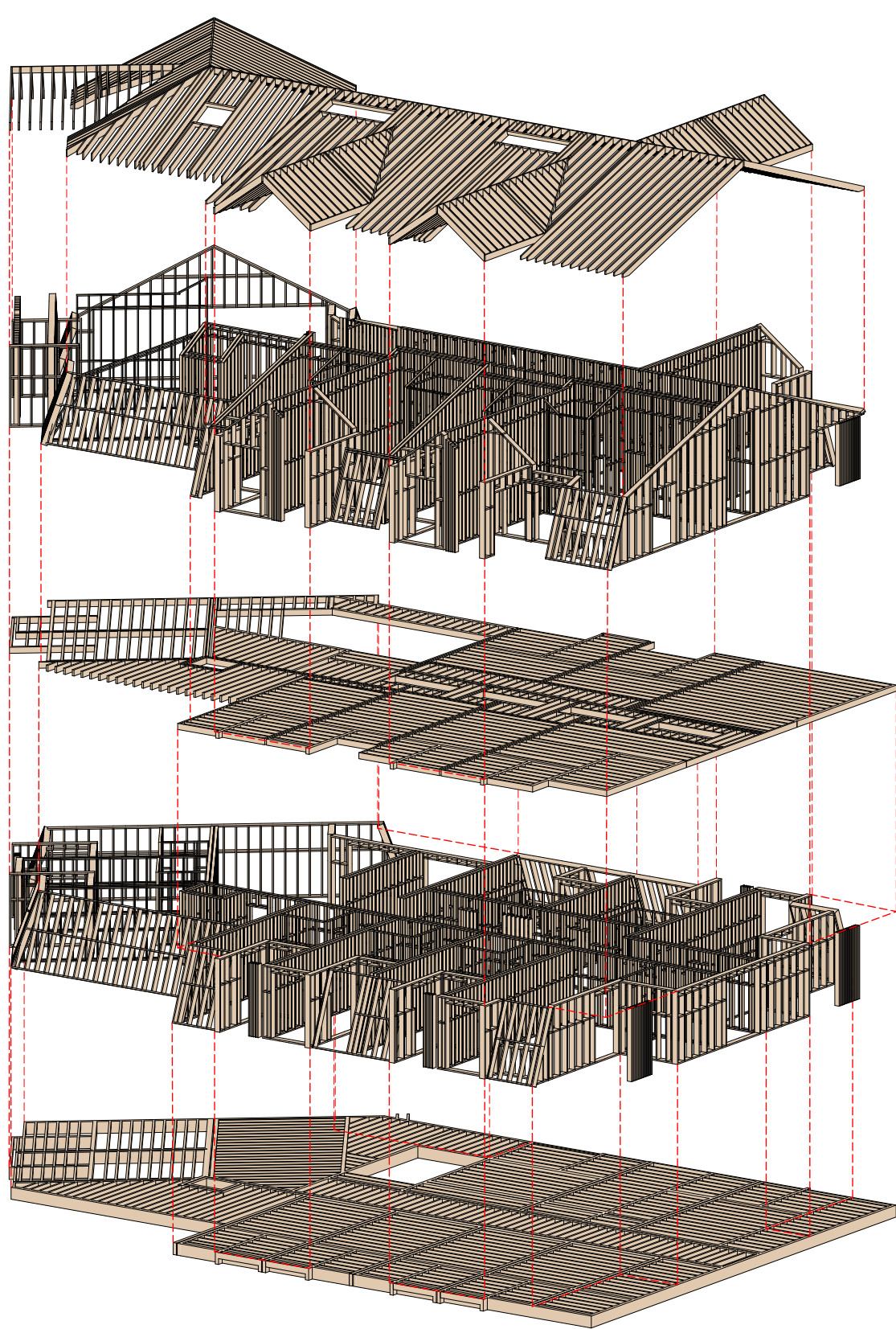
Exploded axonometry - ArchiCAD
