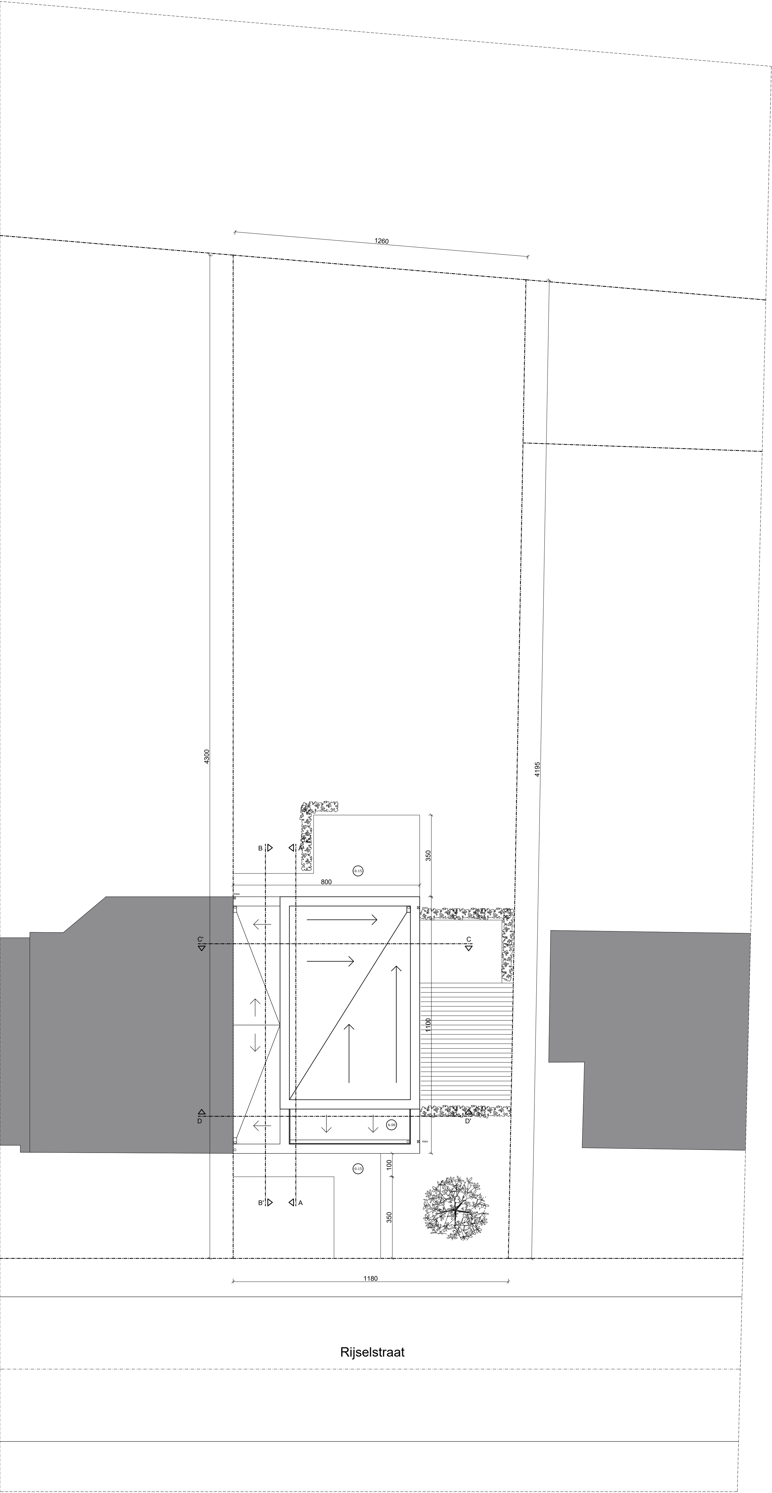
Inplantingsplan
