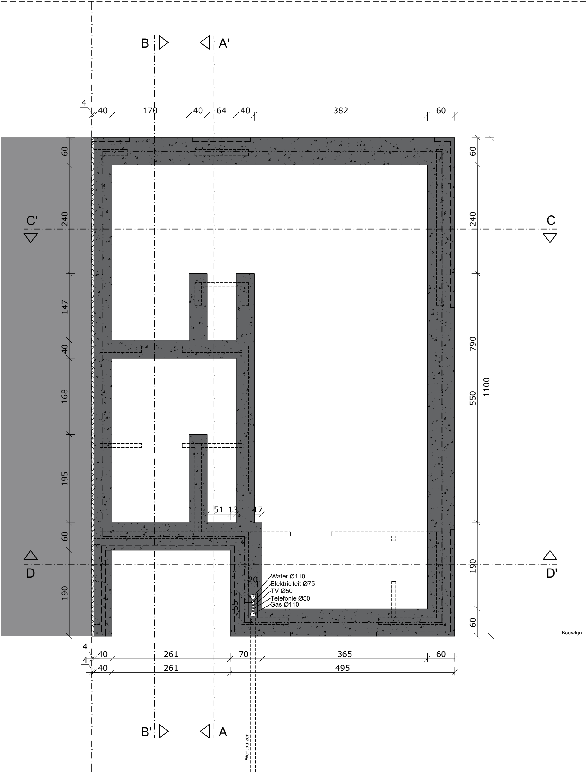
Funderingsplan
